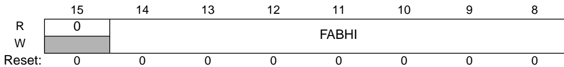
Figure 3-10 fts128k: Flash 8-bit Address High Register (FADDRHI)
